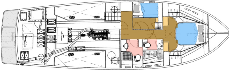
LAYOUT: Main and Lower Deck – Saloon, Galley, Pilothouse
